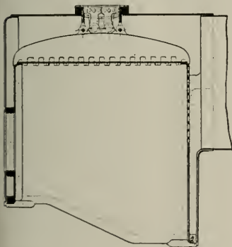
METHOD OF STAYING CROWSHEET, ORLEANS RAILWAY.
